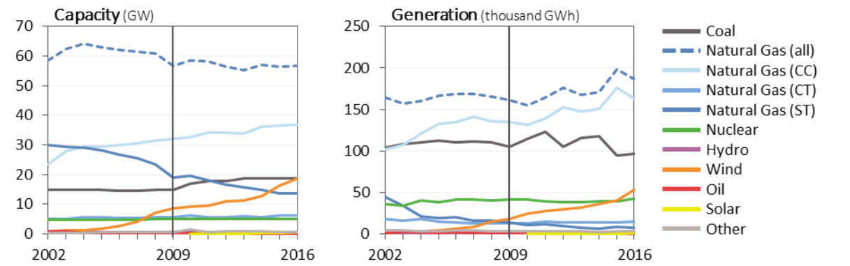
Capacity & Generation by Energy Source, 2002 & 2016
