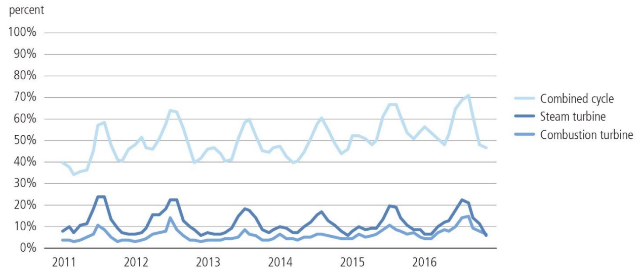
Figure 3.11. Natural Gas Fleet Capacity Factors 54
