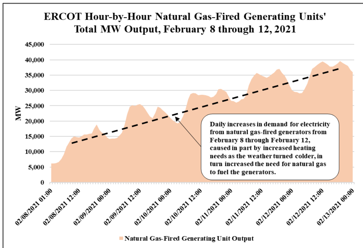
Figure 41: Natural Gas-Fired Generating Unit Production, February 8-12, 2021
