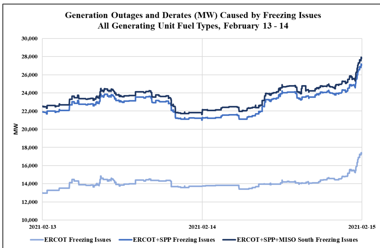
Figure 65: Generation Outages and Derates Due to Freezing Issues – February 13 - 14
