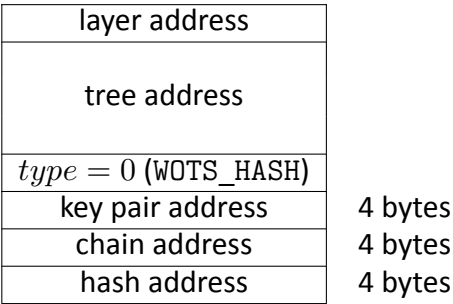
Figure 3. WOTS + hash address
