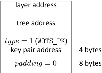
Figure 4. WOTS + public-key compression address
